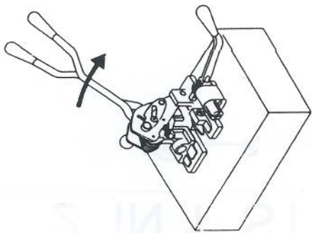
1 Position tool on carton with crimping handle raised back.
