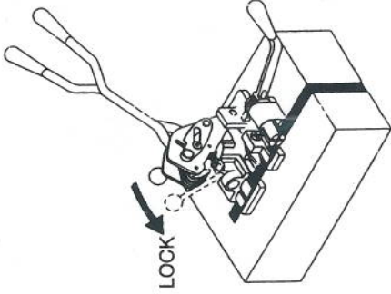
3 Lock strapping into place.
