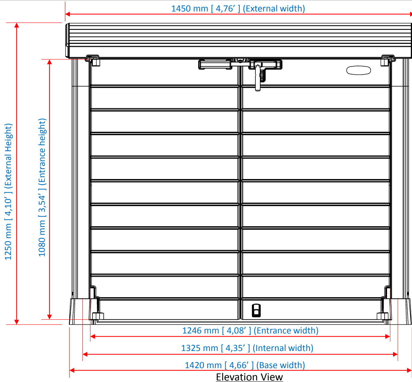
1200L Storage shed (Flat lid)
