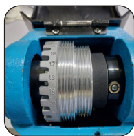
Indexation 24 positions
