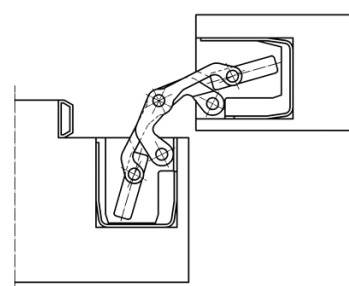
Blockzarge 90°
