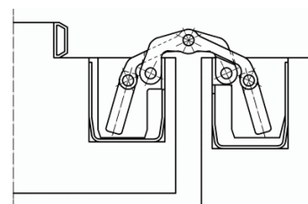
Blockzarge 180°
