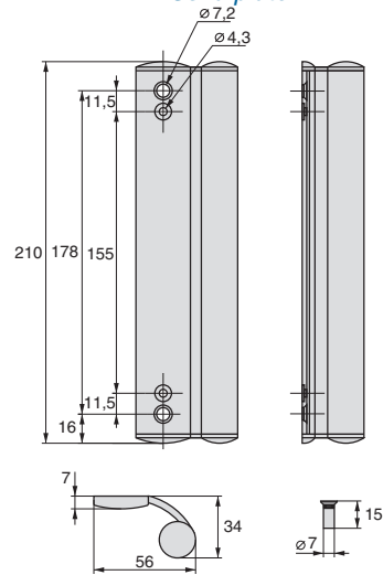
Plaque borgne 6406 Solid plate
