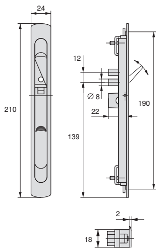
Cuvette levier 6401 Lever handle pan
