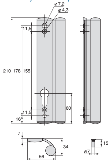
Plaque trou cylindre 6405 Cylinder hole plate
