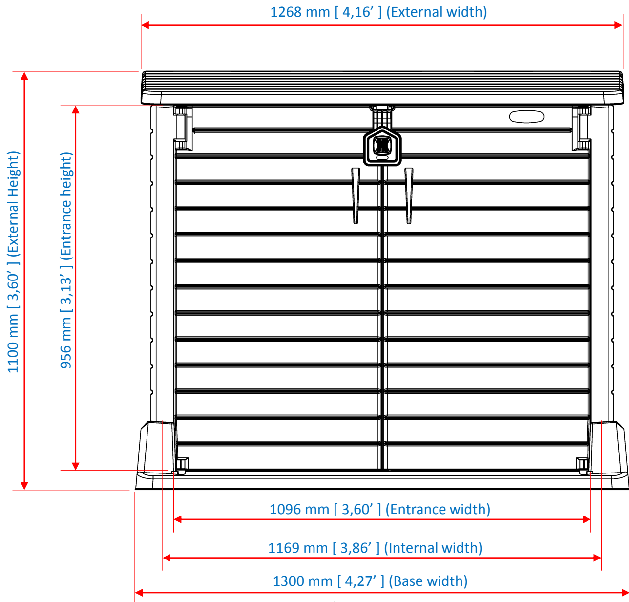
Elevation View
