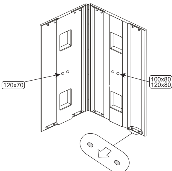
MONTAGE A GAUCHE/ LEFT ASSEMBLING/ MONTAGE LINKS
